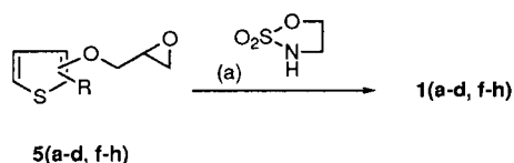
Scheme 2. Route II. (a) NaOH, 50°C, 1 h.
