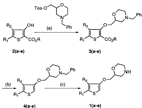
Scheme 1. Route I. (a) DMF, 150°C, 17 h; (b) NaOH, \Delta , 1 h; (c) (i) PdCl_2 , C, H_2O , (ii) MeOH, [H_2] , 1 atm.
