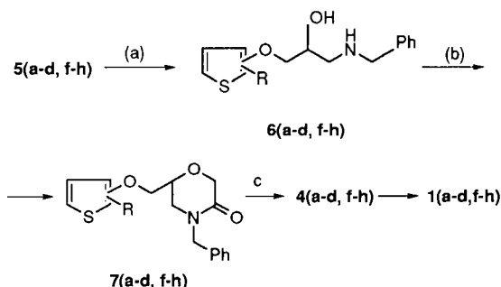
Scheme 3. Route III. (a) Benzylamine, 100°C, 30 min; (b) (i) Et_3N , ClCH_2COCl , (ii) Na/MeOH, \Delta , 8 h; (c) H_4LiAl , \Delta , 6 h.
